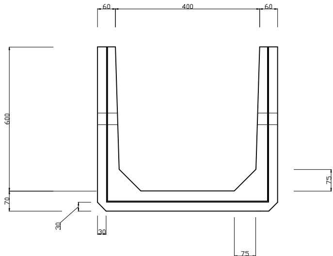
FRONT VIEW SCALE 1: 15
