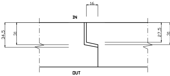
DETAIL JOINT
