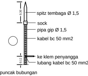
DETAIL SPITZ SKALA 1: 25
