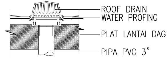
DETAIL ROOF DRAIN skala 1 : 10
