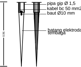
DETAIL ELECTRODA PENTANAHAN SKALA 1:25
