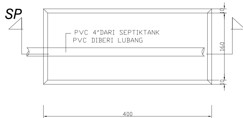
DETAIL RESAPAN
