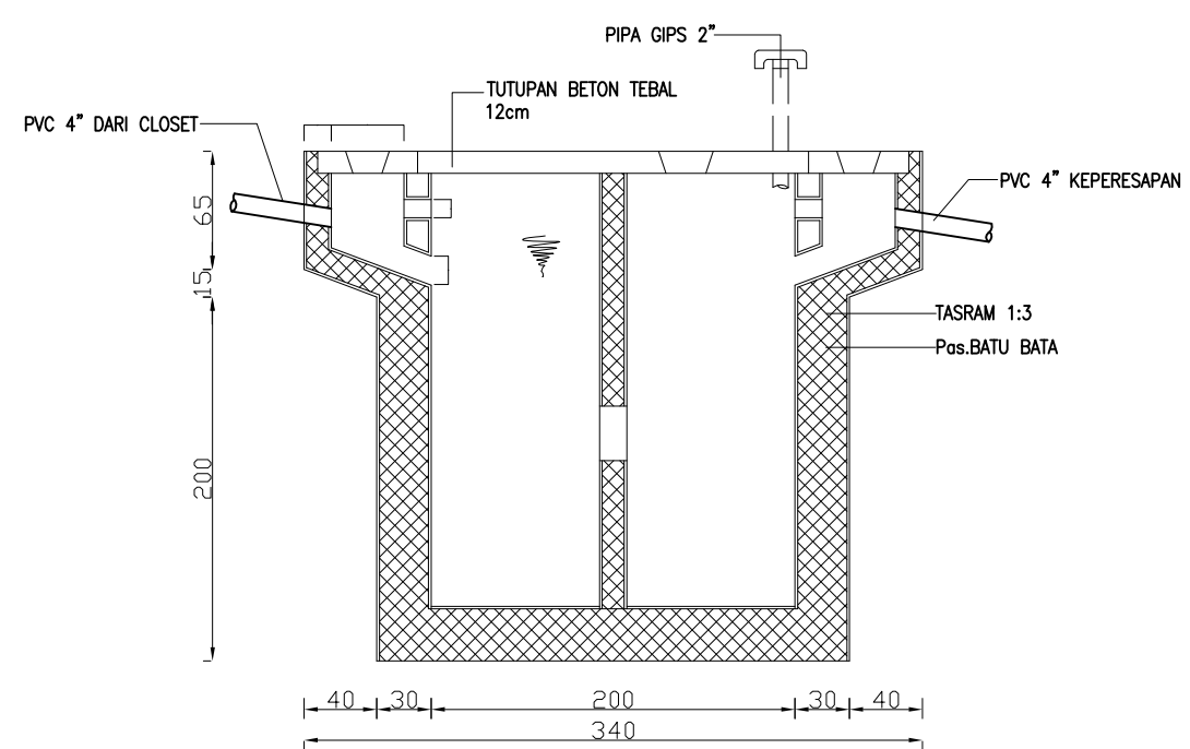
DETAIL SEPTICTANK skala 1 : 25
