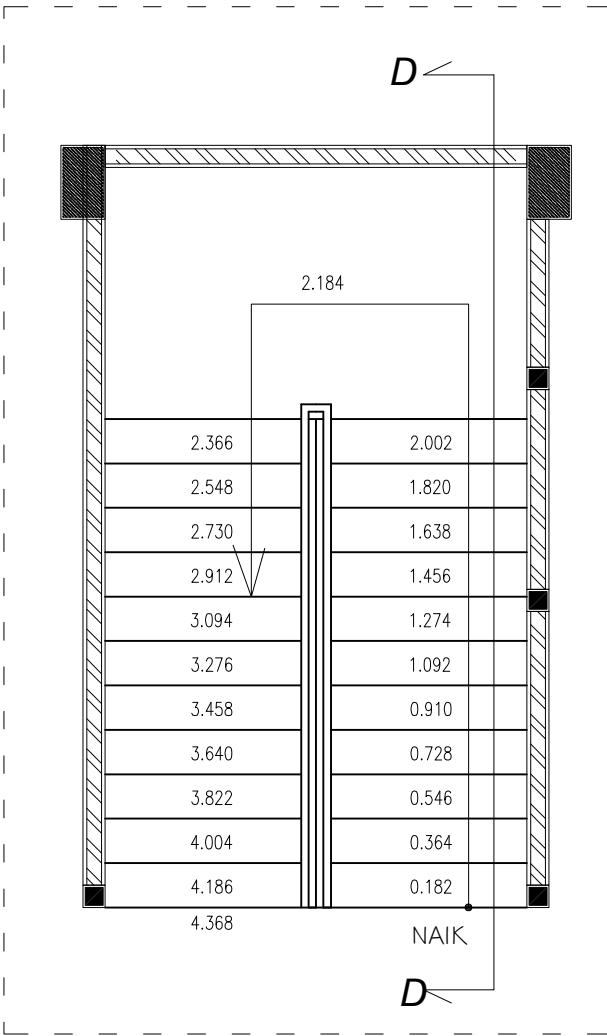
DENAH TANGGA
